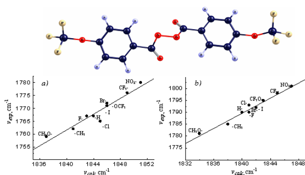
Fig. 3 - Structural model of (4-CF 3 O-C 6 H 4 -COO) 2 (PM6 method) and dependence of the normal antisymmetric (a) and symmetric (b) vibration frequencies of carbonyl groups obtained experimentally ( \nu_{exp} ) and calculated by the PM6 method ( \nu_{calc} ) for the benzoyl peroxide derivatives
