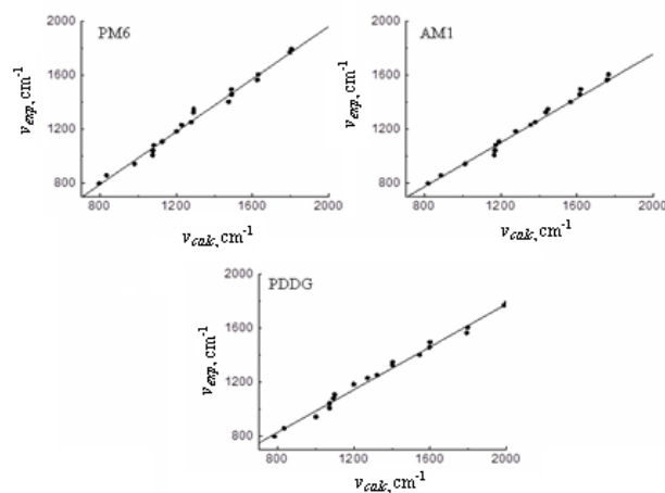
Fig. 2 - Relationships between the experimental (ν exp ) and calculated (ν calc ) normal vibrations frequencies of the benzoyl peroxide IR spectrum in CH 2 Cl 2 (CPCM solvation model)
