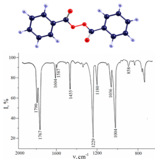
Fig. 1 - Structural model of the benzoyl peroxide (PM6 method) and its experimental IR spectrum in CH 2 Cl 2 , [ROOR] = 0.14 mol/dm 3 , thickness 0.058 mm (according to the Ref. [4])
