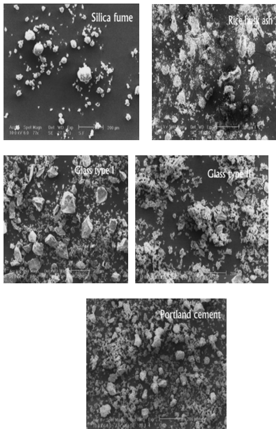
Fig. 2 - Particle size and shape of ground waste glass type I, type II, silica fume, rice husk ash and ordinary Portland cement
