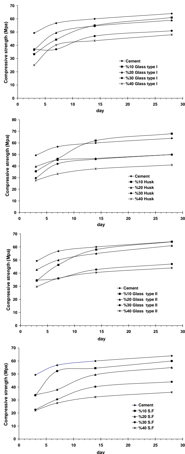
Fig. 3 - Compressive strength test results
