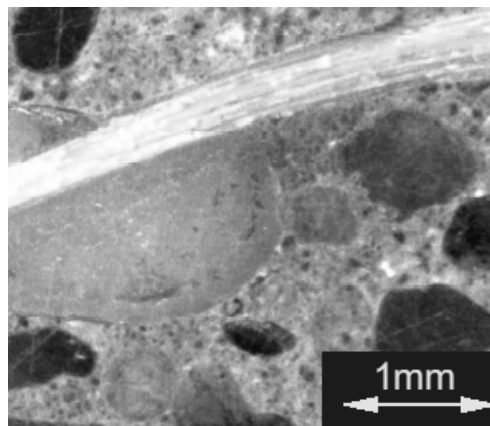
Fig. 4 - Geofiber™ in glasscrete composite
