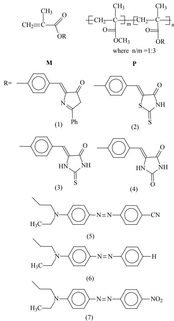
Fig. 1 - The chemical structure of synthesized benzylidene and azo- containing monomers and copolymers.
