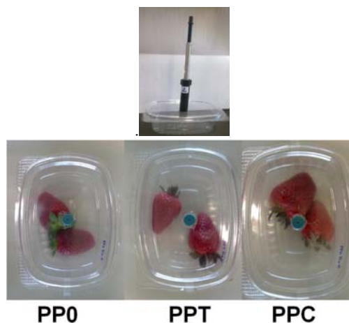
Fig. 1 - Experimental assembly used for headspace analysis of whole strawberries by HS-SPME
