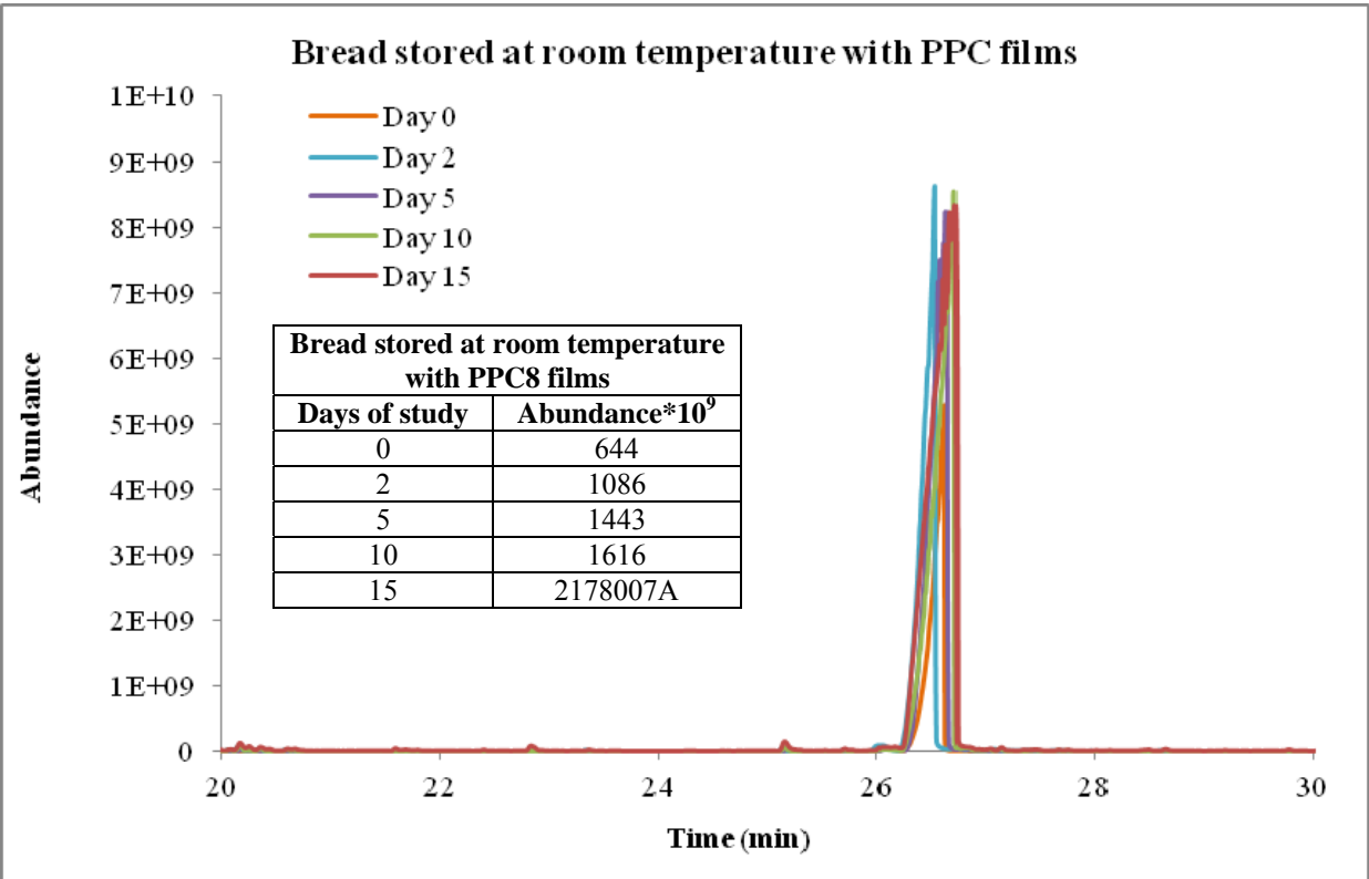
Fig. 4 - Release of carvacrol in the headspace of bread slices after 0, 2, 5, 10 and 15 days of storage at room temperature
