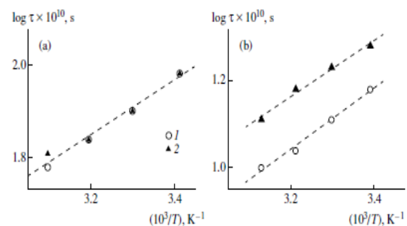
Fig. 3 - The plots of rotation correlation time versus temperature for Tempol radical in the (a) dense and (b) loose regions of (1) textured and (2) isotropic PHB matrices
