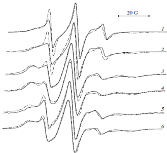
Fig. 2 - EPR spectra of Tempo (1, 2) and Tempol (3–6) radicals in textured (1, 3, 5) and isotropic (2, 4, 6) PHB samples in the (1–4) dry and water-saturated (5, 6) state. Dashed curves show the calculated spectra, solid lines present the experimental spectra measured at T = 20^\circ\text{C} . The curves for Tempo (1, 2) were calculated using the following parameters: \tau_1 = 1 \times 10^{-9} s; w_1 = 0.4 (1), 0.25 (2); \tau_2 = 8 \times 10^{-9} s (1), 6 \times 10^{-9} s (2); w_2 = 0.6 (1), 0.75 (2). The parameters used in calculating the curves for Tempol (3–6) are listed in the table
