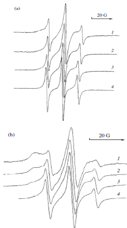
Fig. 1 - EPR spectra of (a) Tempo and (b) Tempol radicals in dry textured PHB films at T = 20 (1); 40 (2); 60 (3); 80°C (4)
