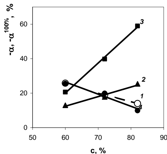
Fig. 2 - (1,4) -\alpha and (2, 3) -\alpha^{100\%} vs. overall content of butadiene units c for (1) EPDM-40, (2) EPDM-60 (II), (3) Elastokam 7505, (4) EPDM R 512 in their covulcanizates with BNR
