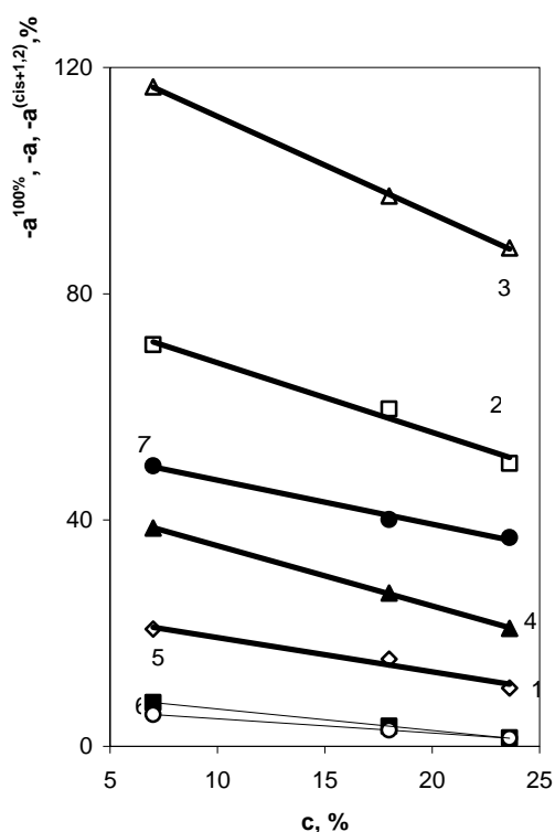
Fig. 1 - The plots the value of -\alpha^{100\%} for covulcanizates EPDM with DSM (1) 778, (2) 714, (3) 712, (7) EPDM-60(I); -\alpha (4) for R 521; -\alpha^{cis+1,2} for (5) R 505 and (6) Elastokam 6305 as a function of the total content of 1,4- cis - and 1,2-butadiene isomers in BNR
