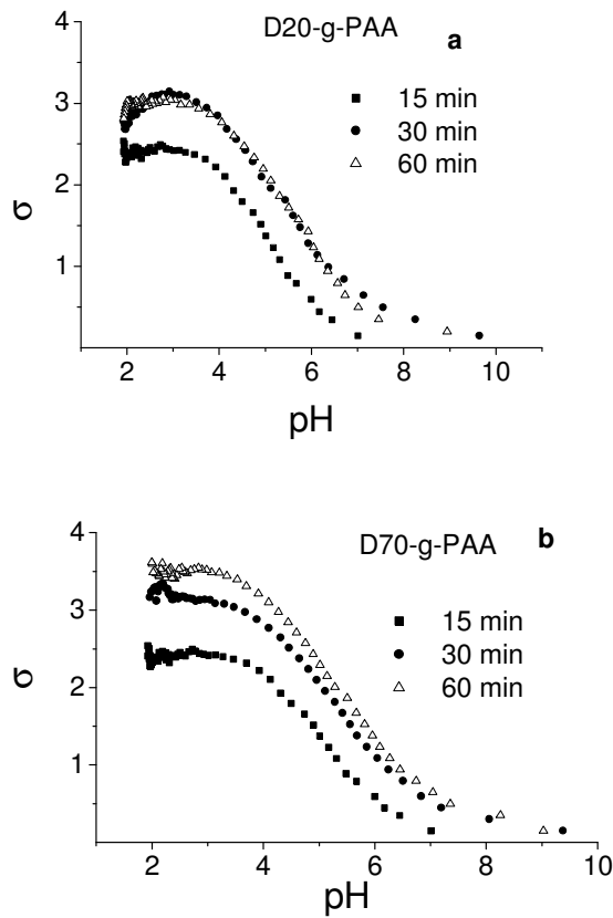
Fig. 4 - Dependence of H^+ absorbance degree on pH for modified D20-g-PAA samples (a) and D70-PAA (b) in 15, 30, 60 min of alkaline hydrolysis
