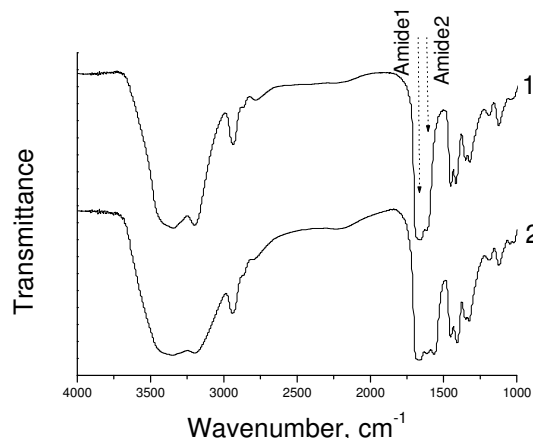
Fig. 3 - FTIR spectra of nonionic (1) and modified (2) D20-g-PAA samples
