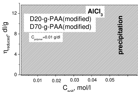
Fig. 9 - Dependence of reduced viscosity on concentration \text{AlCl}_3 for modified D20-g-PAA and D70-g-PAA samples (time of hydrolysis 15, 30 and 60 min)
