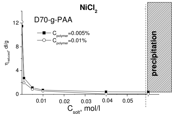
Fig. 7 - Dependence of reduced viscosity on concentration NiCl_2 for modified D70-g-PAA samples (time of hydrolysis 30 min)
