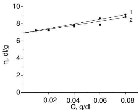
Fig. 2 - Dependence of reduced viscosity on the concentration for D20-g-PAA (1) and D70-g-PAA (2)
