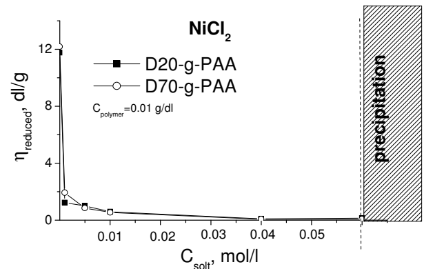
Fig. 8 - Dependence of reduced viscosity on concentration NiCl_2 for modified D20-g-PAA and D70-g-PAA samples (time of hydrolysis 30 min)
