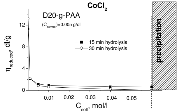
Fig. 6 - Dependence of reduced viscosity on concentration CoCl_2 for modified D20-g-PAA samples
