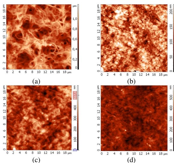
Fig. 1 - AFM topographic images of PHB films (170 kDa) with a scan size of 18x18 \mu\text{m} : the rough surface of fresh-prepared sample (exposed to air) – (a); the smooth surface of fresh-prepared sample (exposed to glass) – (b); the sample exposed to phosphate buffer at 310K for 83 days – (c); the sample exposed to phosphate buffer at 343K for 83 days – (d) General magnification is 300 [17]
