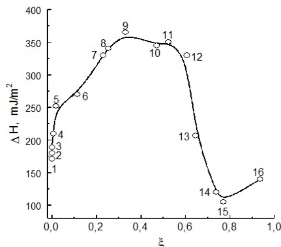
Fig. 3 - The heat of CB No. 254 wetting by liquids versus the polarity of a liquid. Carbon tetrachloride (1), n-hexane (2), 2,2,4 - trimethylpentane (3), ethylbenzene (4), toluene (5), 1 - chlorobutane (6), MMA (7), tetrahydrofuran (8), ethylacetate (9), hexanol - 1 (10), dimethylformamide (11), acetonitrile (12), ethanol (13), ethylene glycol (14), glycerin (15), water (16)
