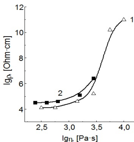
Fig. 1 - \rho of the (PE+CB)+PMMA (1) and (PS+CB)+PE (2) systems versus the effective viscosity of PMMA and PE correspondingly. Concentration of CB: 5.4 vol. % in the PE phase (1), 9.3 vol. % in the PS phase (2)
