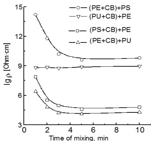
Fig. 4 - \rho of polymer blends versus time of mixing. The CB content: 5 vol. % in the PE phase, 8.5 vol. % in the PU phase, 9.3 vol. % in the PS phase. The ratio of polymers is 1:1
