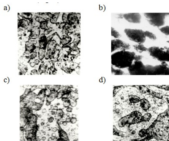
Fig. 2 - Distribution of CB in the blends: (PE+CB)+PU (a); (PU+CB)+PE (b), (PS+CB)+PE (c), (PE+CB)+PDMS (d) filled with 2.5 vol. % CB (Optical micrograph). The ratio of polymers is 1:1. Taking the components in brackets means their premixing. Magnification: 1100
