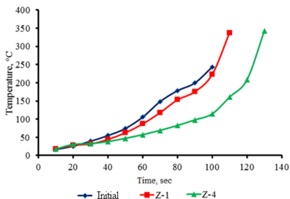
Fig. 2 - Dependence of temperature on the unheated sample surface on the heating time
