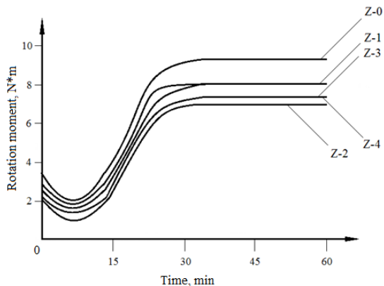
Fig. 1 - Kinetic curves of vulcanization: 1 – Control rubber mixture Z-0; 2 - mixture Z-1; 3 - mixture Z-2; 4 - mixture Z-3; mixture Z-4
