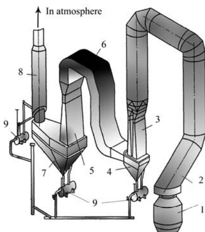
Fig. 5 – The scheme of clearing of flue gas with gas cooling in a Venturi scrubber and the subsequent clearing in a rotoklon: 1 - baking oven; 2 - gas exit branch; 3 - Venturi scrubber; 4 - bunker - the drop catcher; 5 - rotoklon; 6 - gas pipeline; 7 - inertial heat - and a mist eliminator; 8 - exhaust pipe; 9 - tank - a hydraulic hitch
