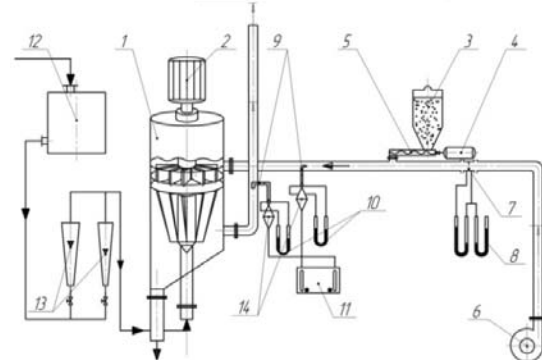
Fig. 2 – the Circuit design of experimental installation: 1 - scrubber; 2 - the drive; 3 - the dust loading pocket; 4 - the electric motor; 5 - the batcher; 6 - the fan; 7 - a diaphragm; 8,10 - differenti 12 - the pressure tank; 13-rotametr; 14 - sampling instruments
