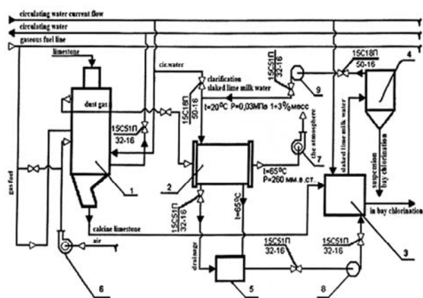
Fig. 6 – Flowchart of clearing of gas emissions
