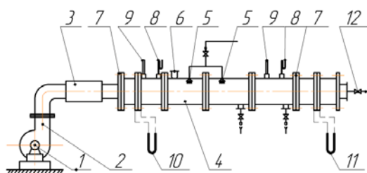
Fig. 3 – The Circuit design of experimental installation: 1 - electric motor; 2 - ventilating fan; 3 - hot-air heater; 4 - the whirlpool chamber; 5 - atomizers; 6 - loading pocket; 7 - diaphragm; 8,10 - differential pressure gauges; 9 - the thermometer; 11 - the fine gauge strainer; 12 - the coincidence gate
