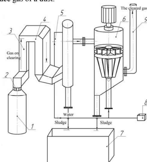
Fig. 4 – Process flowsheet of clearing of gas emissions: 1 - bake roasting; 2 - water block; 3 - raiser; 4 - downtaking duct, 5 - centrifugal scrubber; 6 - scrubber dynamic; 7 - forecastle of gathering of sludge, 8 - hydraulic hitch, 9 – chimney
