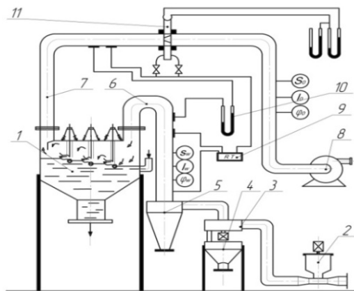
Fig. 1 – The Circuit design of experimental installation: 1-rotoklon; 2 - the dust 2-batcher; 3 - qualifier; 4 - collector of a coarse dust; 5 - cyclone; 6,7-gas pipeline; 8 - the ventilating fan; 9 - potentiometer; 10 - differential pressure gauge; 11 - diaphragm
