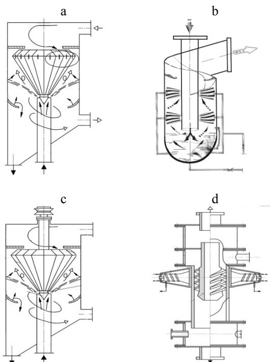
Fig. 8 – The modified variety of apparatuses scrubber under patents for inventions: a) Patent decision № 2012153318/15; b) Patent decision № 2012157446/15; c) № 2339435; d) № 2482923
