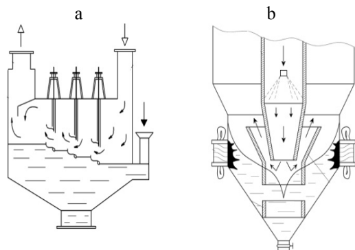
Fig. 9 – The modified variety of apparatuses "Rotoklon" under patents for inventions: a) № 2317845; b) The request №2007120000
