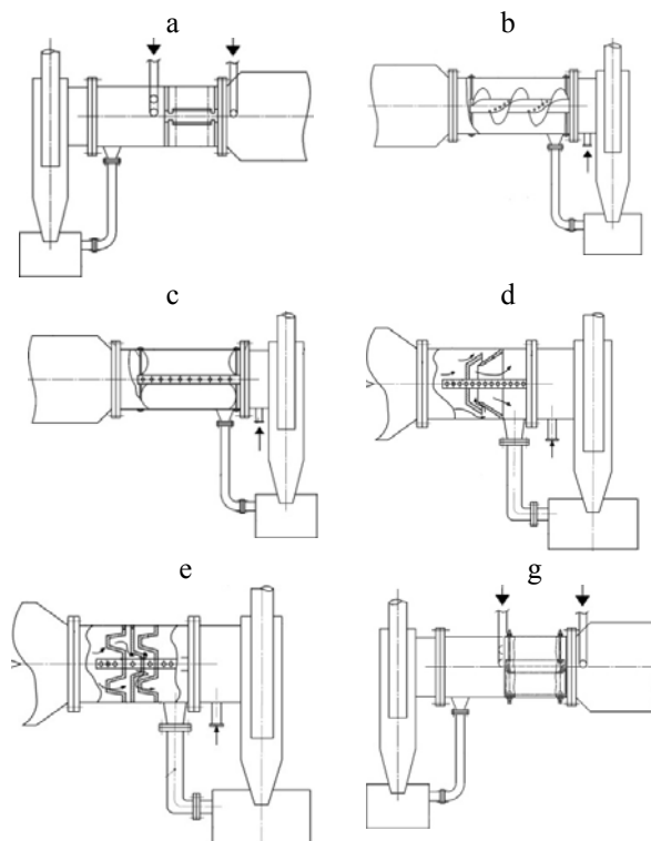
Fig. 7 – The modified variety of apparatuses under patents for inventions: a) №2182843; b) № 2305457; c) № 316383; d) № 2382680; e) № 2403951; g) № 2234358
