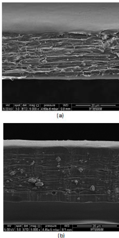
Fig. 4 - SEM micrographs of the cross sections of the film in a) Machine direction, b) Transverse direction
