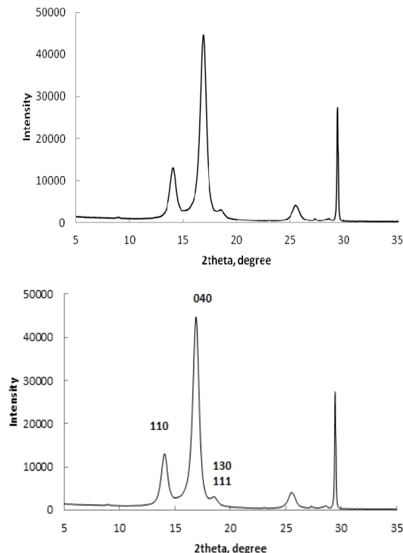
Fig. 2 - X-ray diffraction diagram of the film in 5-35^\circ 2\theta range
