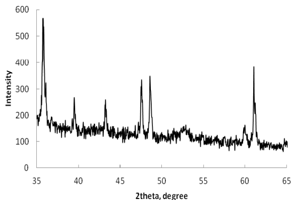
Fig. 3 - X-ray diffraction diagram of the film in 35-65° 2theta range
