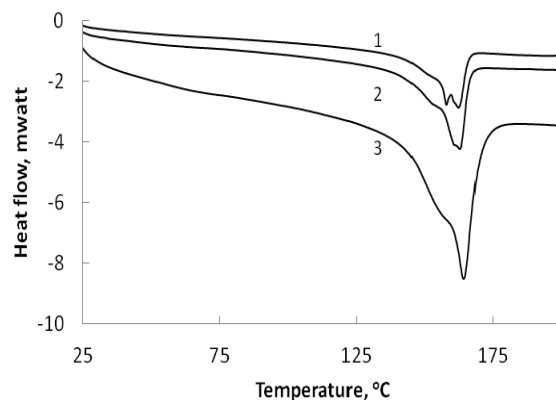
Fig. 6 - DSC curves of the film at 1. 5oC/min, 2.10oC/min, 3. 15oC/min heating rates
