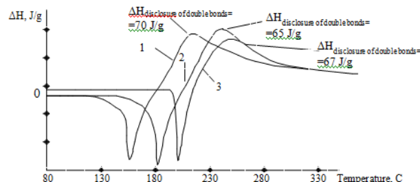
Fig. 1 - DSC curves of BMI: 1 – N,N'-diphenylmethane-bis-maleinimide; 2 – N,N'-diphenyloxide - bis-maleinimide; 3 – N,N'-m-phenylene-bis-maleinimide (FBMI)
